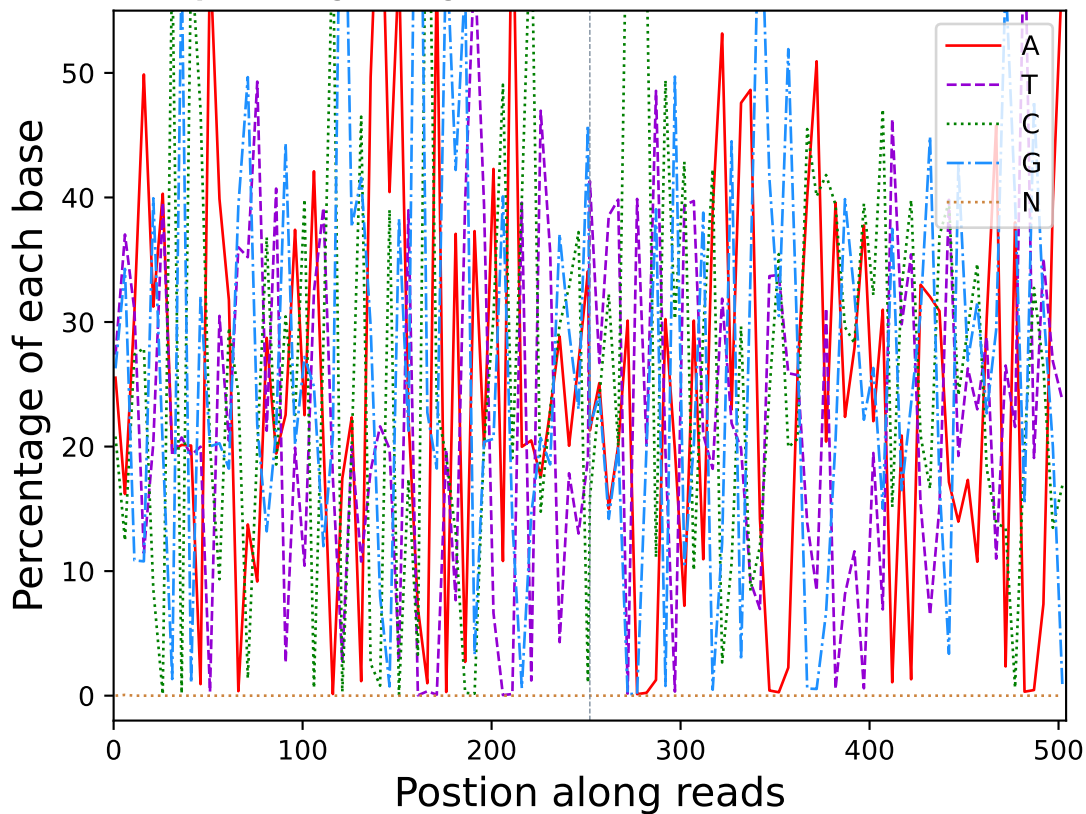
Base percentage along reads (R20112)
